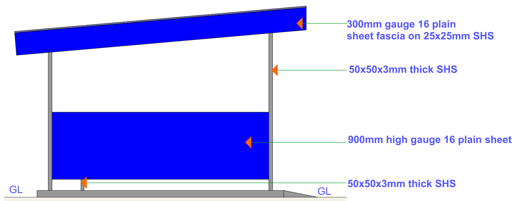
SIDE 02 ELEVATION
