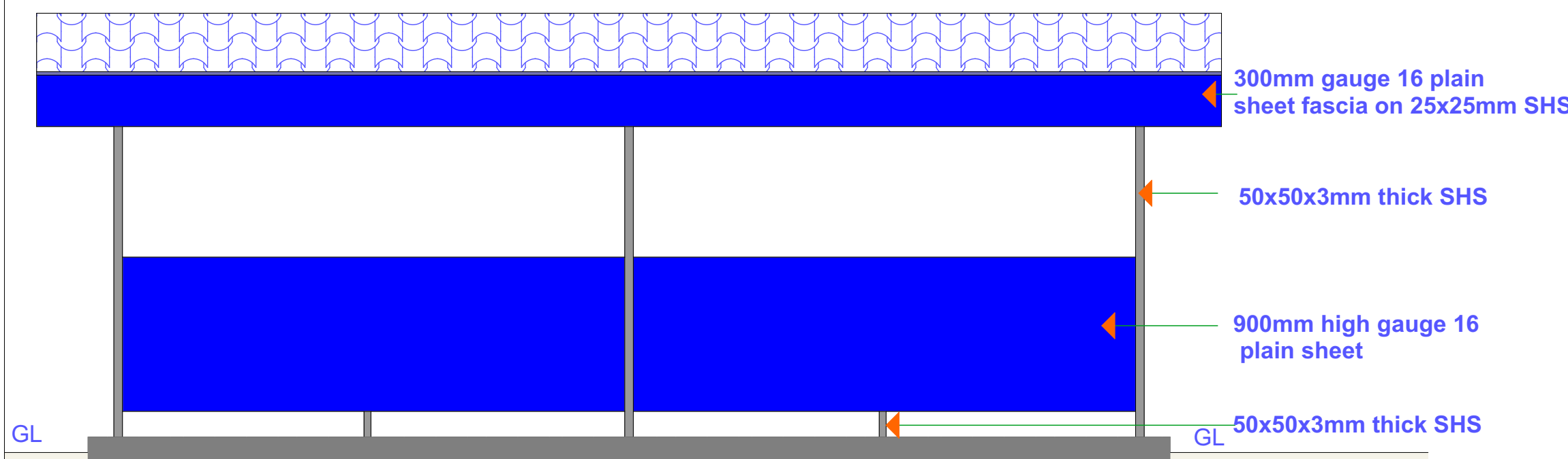
BACK ELEVATION
