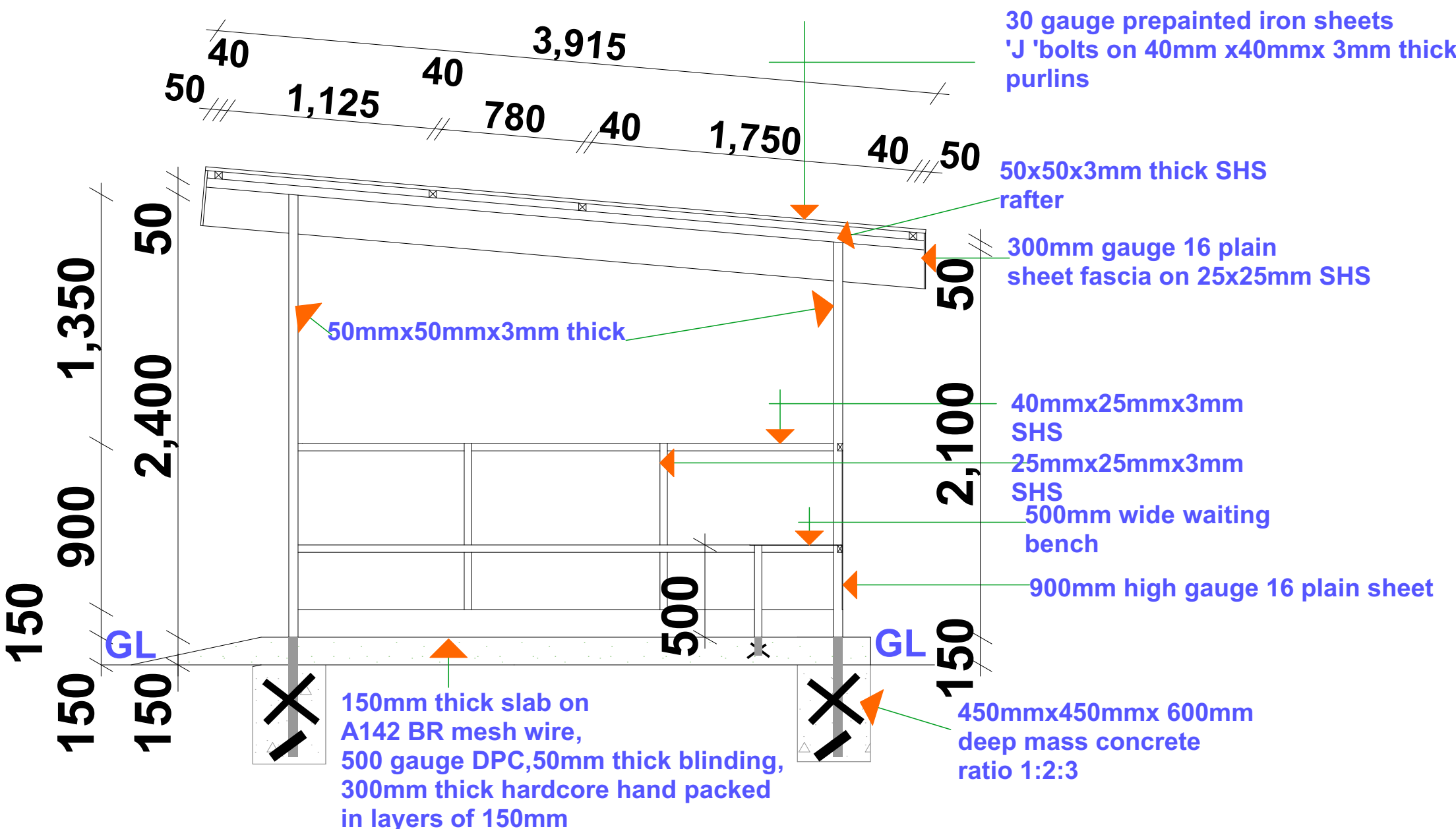
SECTION X
