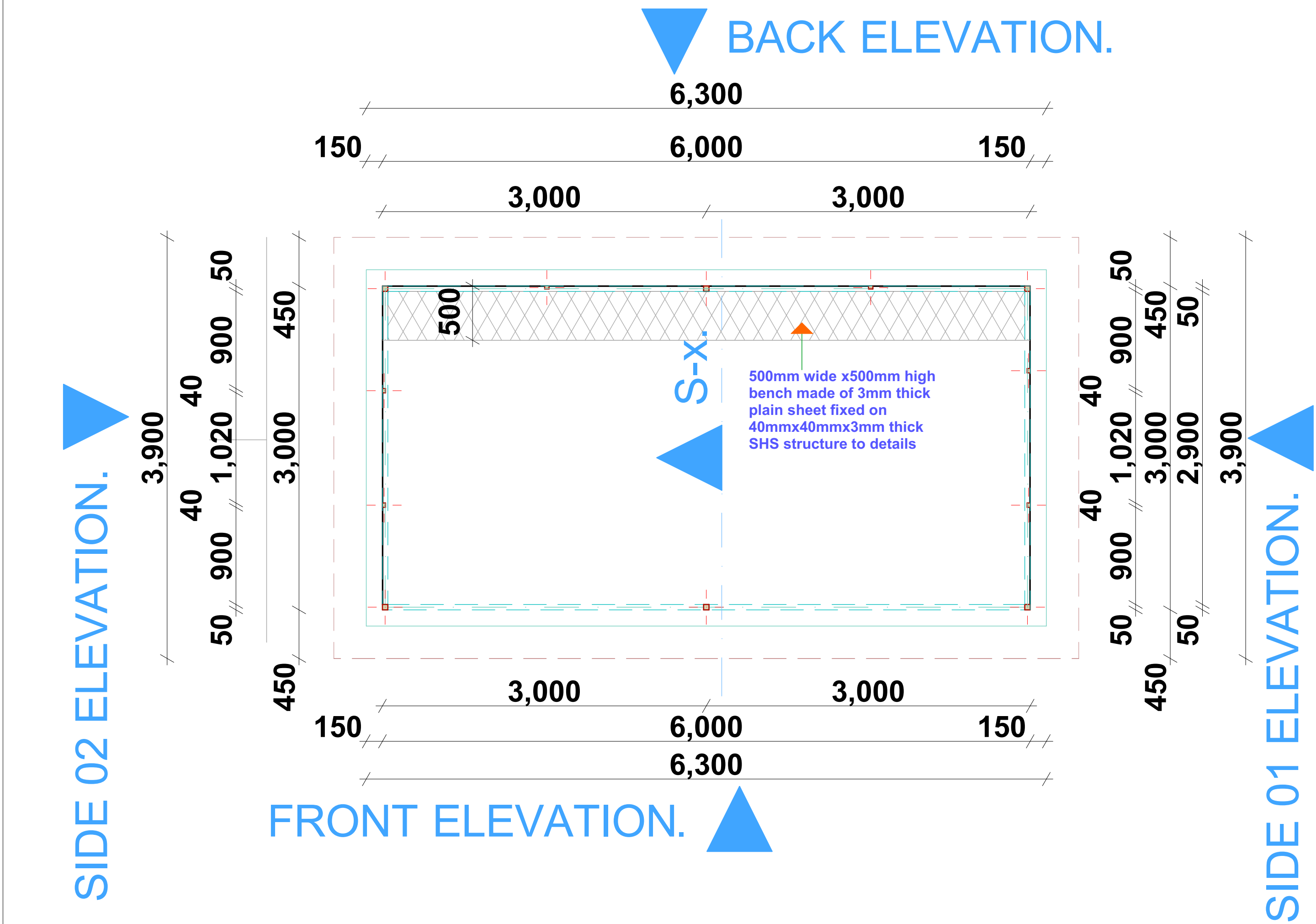
FLOOR PLAN LAYOUT
