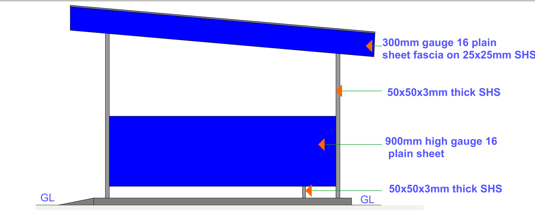
SIDE 01 ELEVATION
