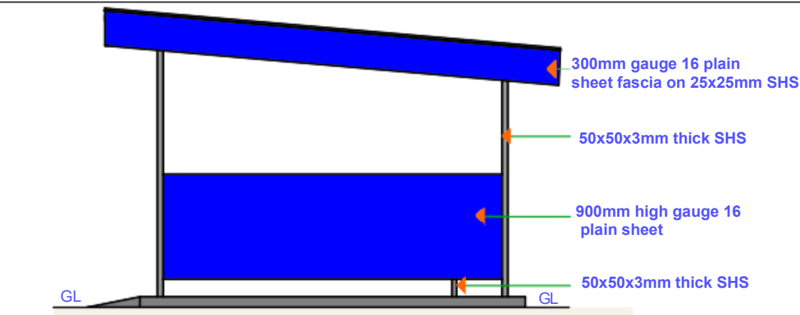
SIDE 01 ELEVATION
