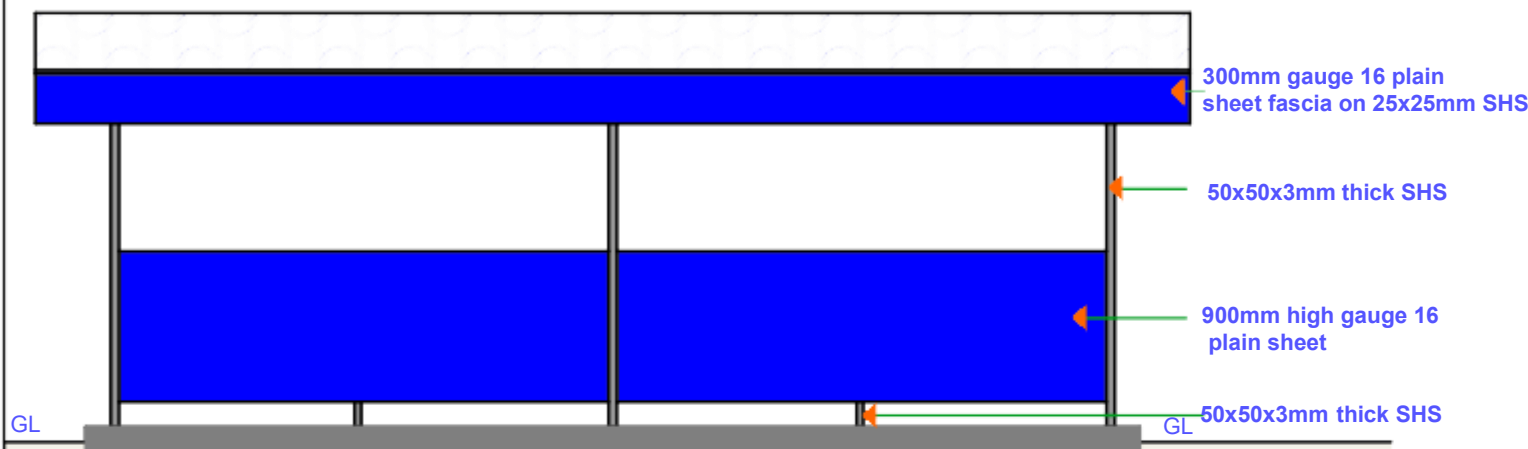
BACK ELEVATION
