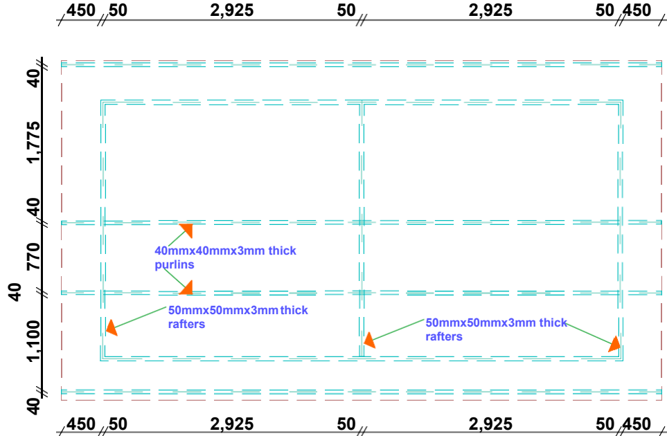
ROOF PLAN
