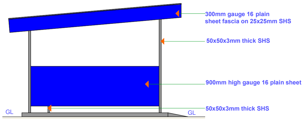
SIDE 02 ELEVATION
