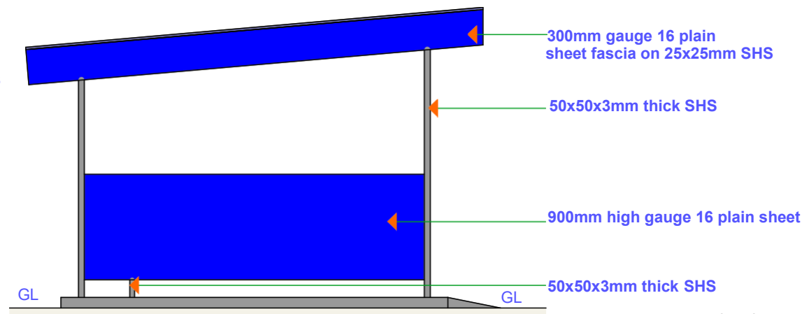
SIDE 02 ELEVATION
