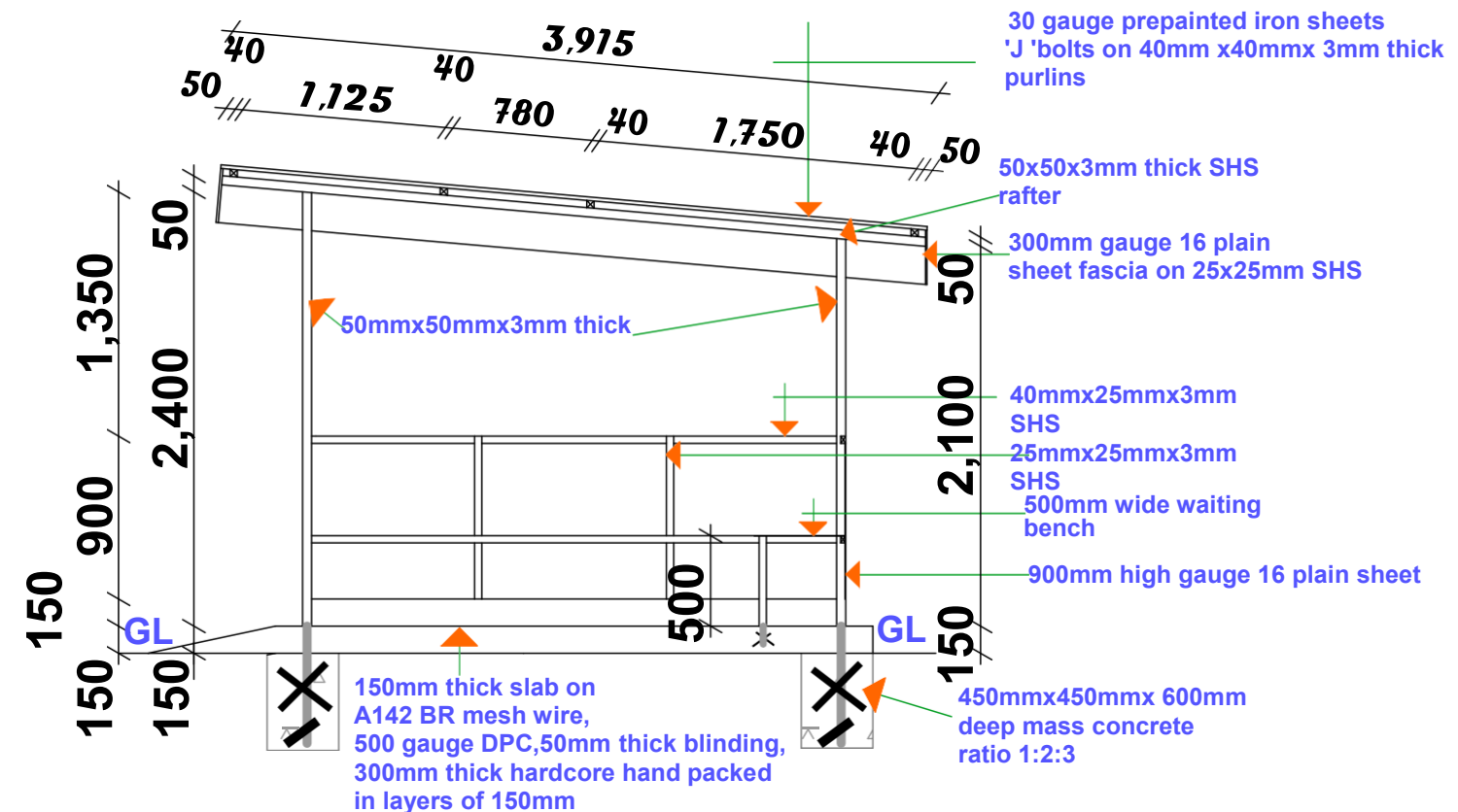
SECTION X
