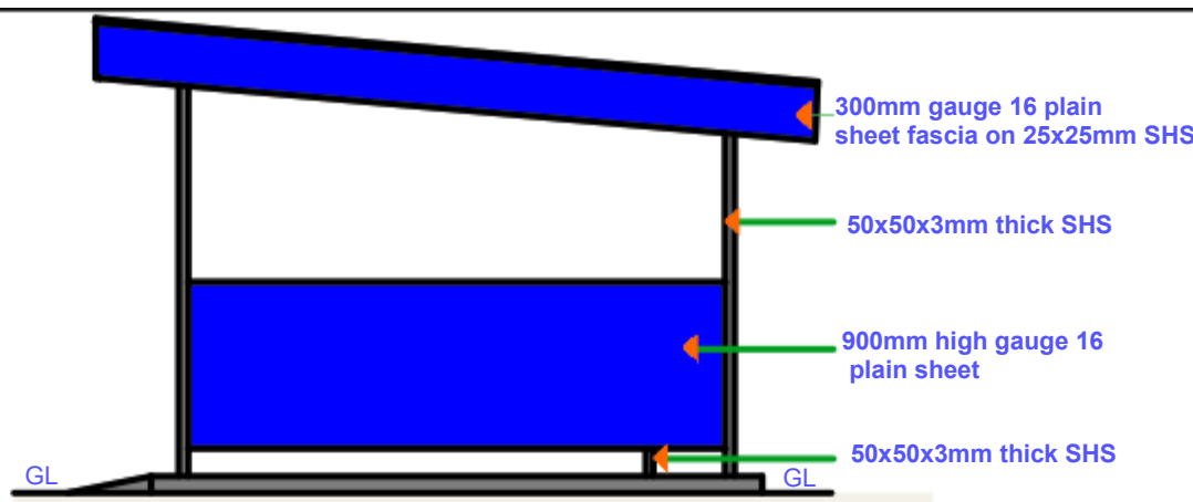
SIDE 01 ELEVATION
