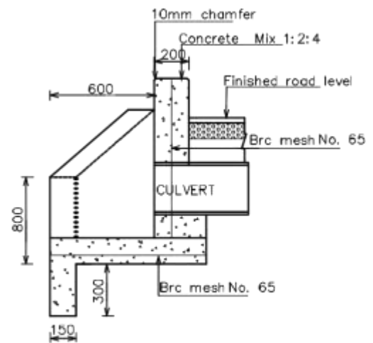
SECTION
