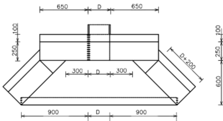
PLAN
